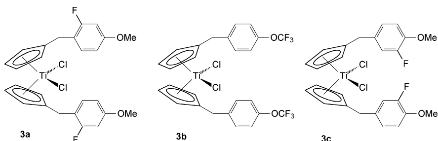
Figure 3. Structures of titanocenes 3a–3c .
