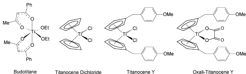
Figure 1. Structures of budotitane, titanocene dichloride, titanocene Y and oxali-titanocene Y.
