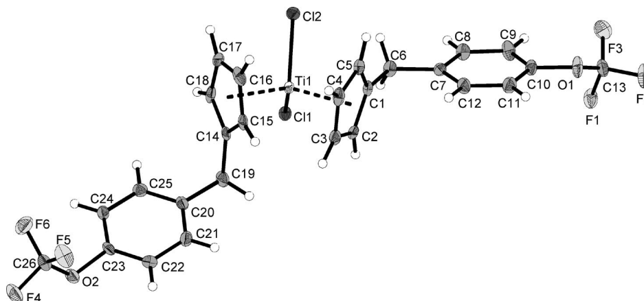
Figure 5. X-ray diffraction structure of bis[4-(trifluoromethoxy)benzyl]cyclopentadienyl}titanium(IV) dichloride ( 3b ); thermal ellipsoids are drawn at the 50% probability level.
