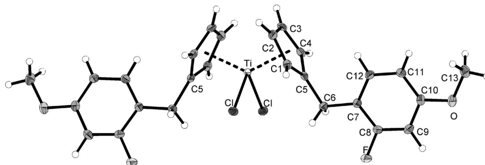
Figure 4. X-ray diffraction structure of bis[(2-fluoro-4-methoxybenzyl)cyclopentadienyl]titanium(IV) dichloride ( 3a ); thermal ellipsoids are drawn at the 50% probability level.
