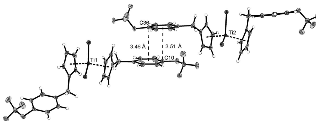
Figure 7. X-ray diffraction structure of two molecules of bis[4-(trifluoromethoxy)benzyl]cyclopentadienyl}titanium(IV) dichloride ( 3c ) connected by \pi - \pi interaction; thermal ellipsoids are drawn at the 50% probability level.
