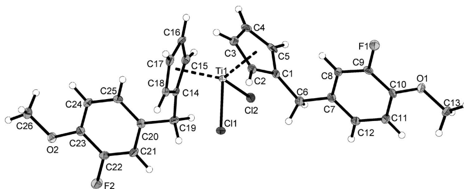
Figure 6. X-ray diffraction structure of bis[(3-fluoro-4-methoxybenzyl)cyclopentadienyl]titanium(IV) dichloride ( 3c ); thermal ellipsoids are drawn at the 50% probability level.
