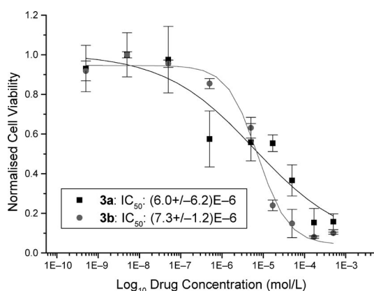
Figure 8. Cytotoxicity curves from typical MTT assays showing the effect of compounds 3a and 3b on the viability of LLC-PK cells.
