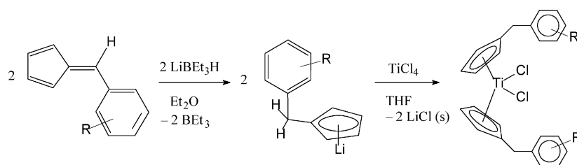
Scheme 1. Synthesis of benzyl-substituted titanocenes from fulvenes by using the hydridolithiation reaction.
