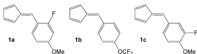
Figure 2. Structures of fulvenes 1a–1c .
